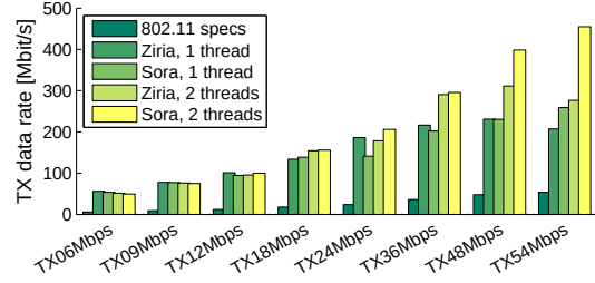
Figure 6: WiFi throughput
