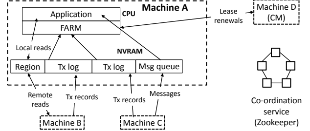
Figure 3. FaRM architecture
