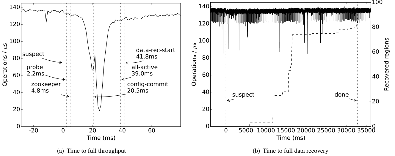
Figure 9. TATP performance timeline with failure
