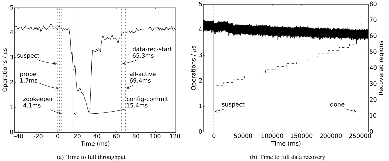
Figure 10. TPC-C performance timeline with failure
