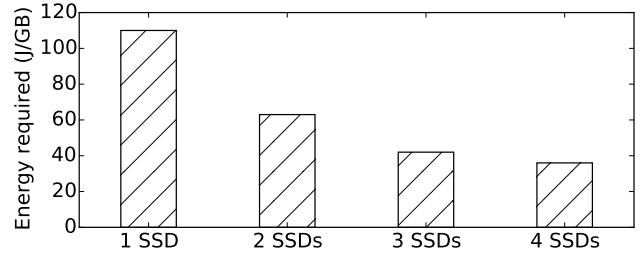
Figure 1. Energy to copy one GB from DRAM to SSD
