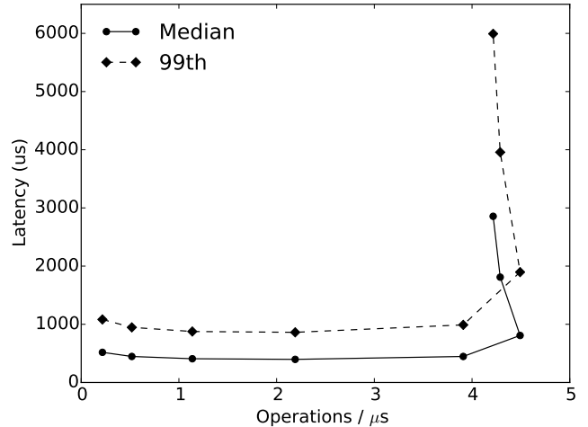
Figure 8. TPC-C performance
