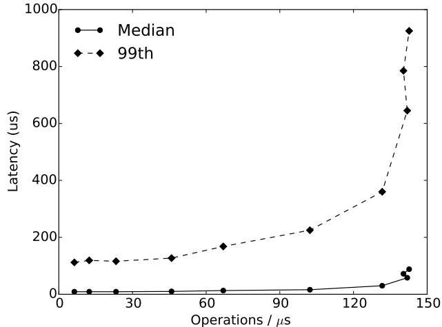
Figure 7. TATP performance
