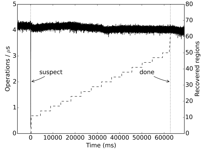
Figure 15. TPC-C throughput with more aggressive data recovery
