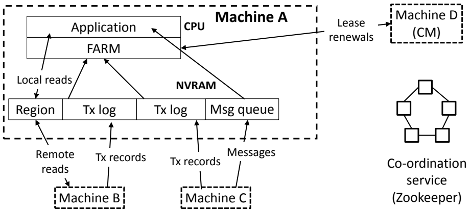
Figure 3. FaRM architecture
