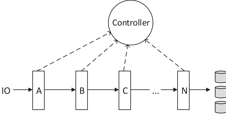
Fig. 11. sSwitches send their measured IO response times for the IO going to file X to the controller.
