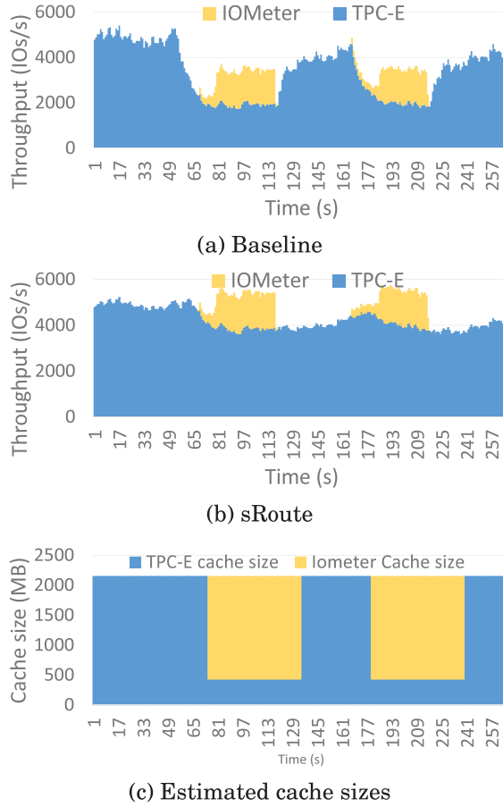
Fig. 10. Maximizing hit rate for two tenants with different cache miss curves.
