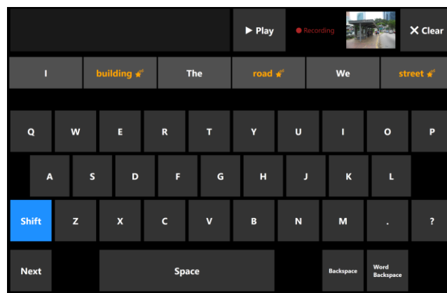
Figure 1. SceneTalk is a gaze-based AAC system that uses the device's camera to recognize objects. Recognized objects are used to suggest relevant words and phrases as the user types. The prediction bar at the top of the keyboard combines contextual predictions detected in the image (in orange) with predictions from a language model (in white).
