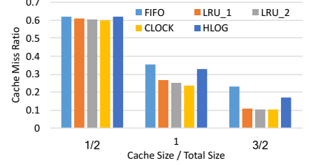
Figure 16: Cache miss ratio (Hot Set).
