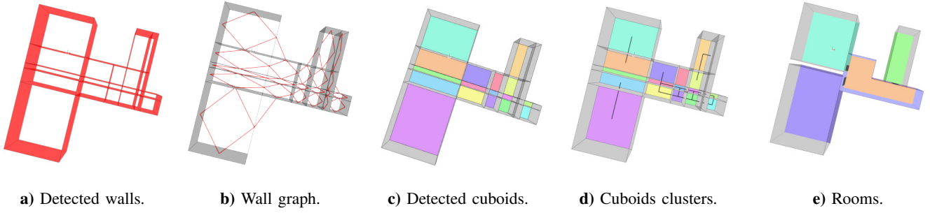
Fig. 4: Room layout detection steps: a) walls detected in previous phase are intersected; b) the wall graph built by iterating through the list of walls in order to analyze wall connectivities; c) connected walls are clustered together to form cuboids; d) the cuboids are clustered based on their connection type; e) cuboids are merged to form rooms.
