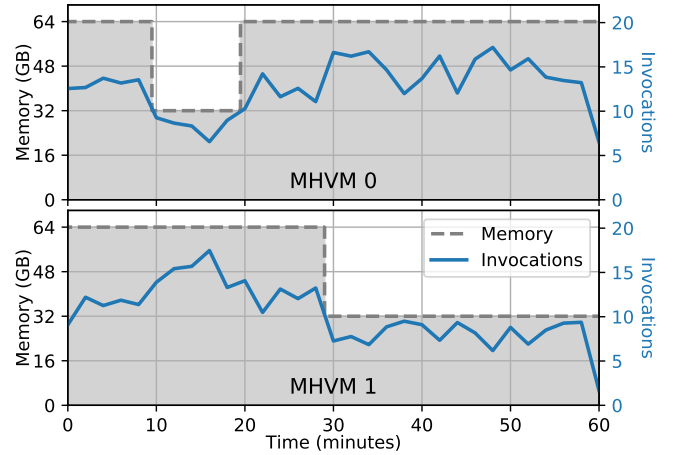
Figure 14: Performance of MH-FaaS running in 2 MHVMs.
