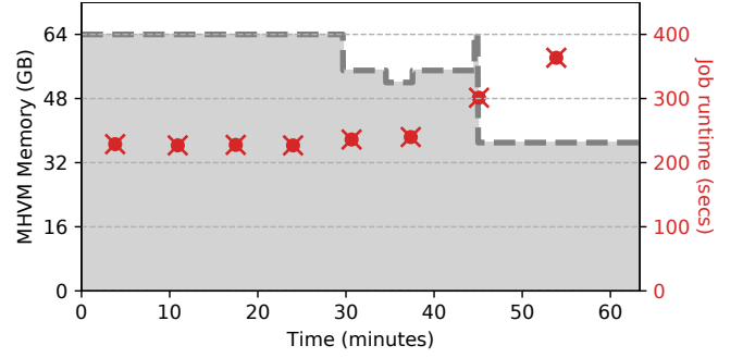
Figure 13: Performance of MH-Hadoop jobs as the MHVM grows and shrinks due to co-located regular VMs arriving and departing.
