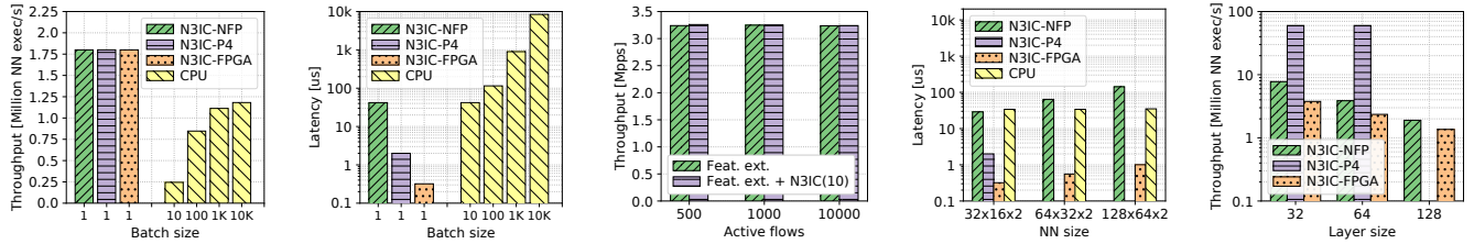
Figure 14: For IoT use cases, N3IC is 1.5x-7x faster than bnn-exec , while N3IC can provide at least 40Gb/s. Figure 15: For Security use cases, N3IC implementations can provide at least 10-100x lower latency than bnn-exec . Figure 16: N3IC-NFP throughput for the IoT use case when analyzing 500, 1k, and 10k parallel TCP flows. Figure 17: N3IC-FPGA can support the network throughput for the IoT tomography use case even in fast 400Gb/s networks with probes sent every 25μs. Figure 18: Maximum throughput in number of BNNs execution per second for N3IC BNN executors.
