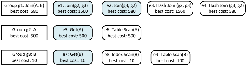
Figure 2.3: An example memo of A \bowtie B , where an index is available on table B . Logical expressions are colored in blue. Physical expressions and groups are annotated with the cost of the corresponding best plans.
