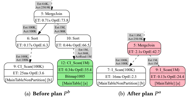
Figure 5: Illustration of regression pattern RP-3.
