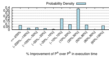
(b) Incremental Index Tuning
